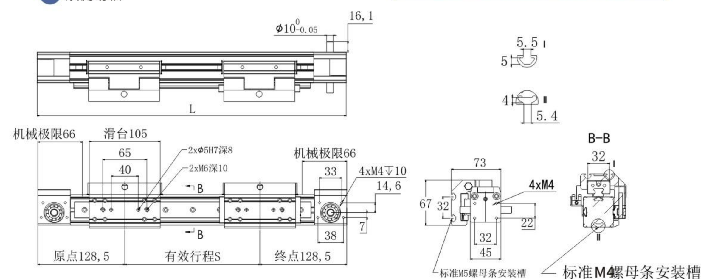
● 双侧动轴
